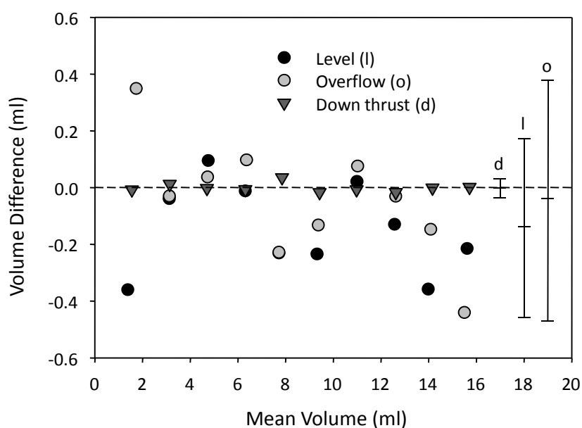
Figure 3. (b) Bland-Altman plots of the data showing the level of agreement between measured and actual volumes. The ‘error bars’ on the right hand side indicate the accuracy (middle bar) and precession (top and bottom bars) of the three techniques. 95% of the data are expected to fall within \pm 1.96\sigma .
