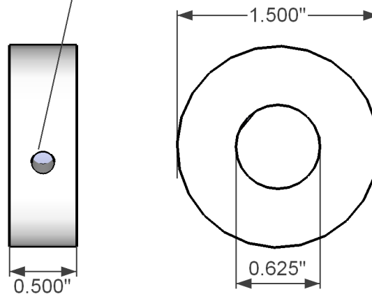
Spindle Thrust Bearing Brass (1 piece)
