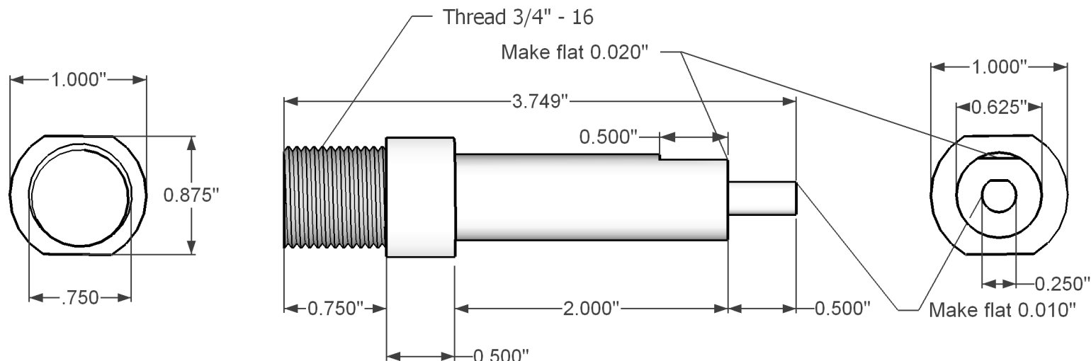
Head Spindle CRS (1 piece)
