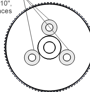
90 Tooth Worm Gear SDP/SI product number: S1C86Z-P048B090S Brass
