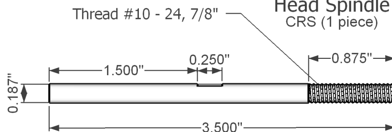
Worm Axle CRS (1 piece)
