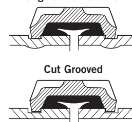
AGS Roll Grooved Grooved
