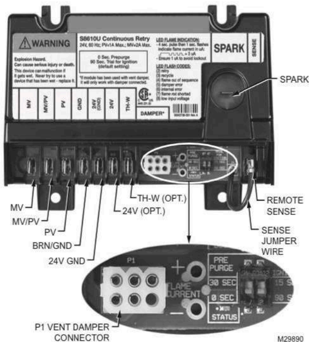
Fig. 1. Typical wiring connections.
