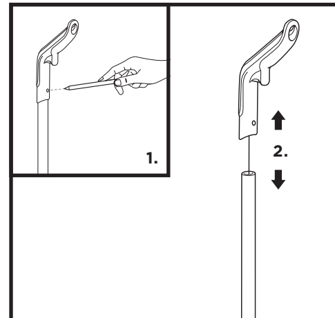
DISASSEMBLE VACUUM HANDLE
